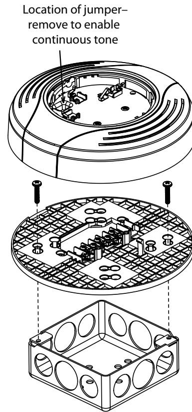
FIGURE 3: MOUNTING
